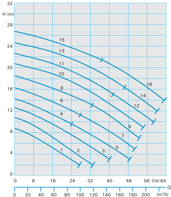
Hydraulic performance
